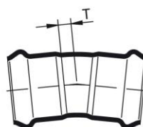
Double socket bend 45°
